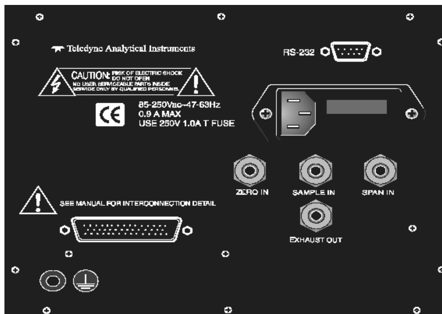
Figure 3-3: Rear Panel of the Model 3000TA-EU
