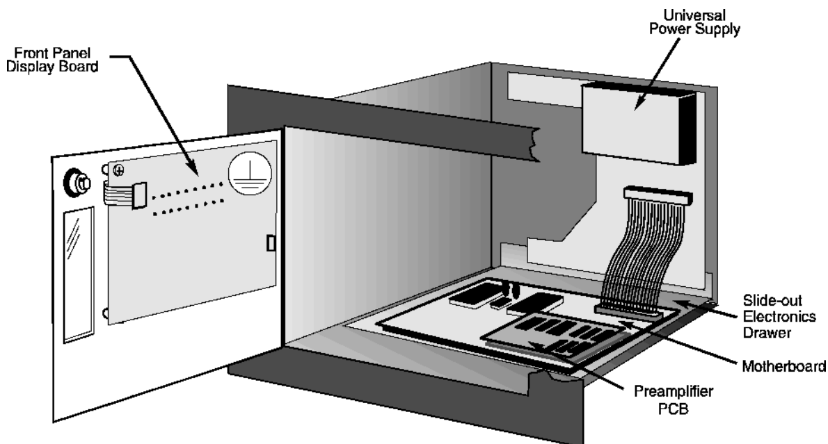
Figure 2-6: 3000TA-EU Internal Electronic Component Location
