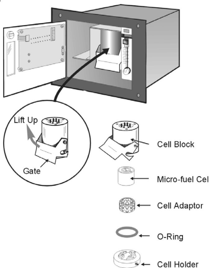
Figure 5-1: Removing the Micro-Fuel
