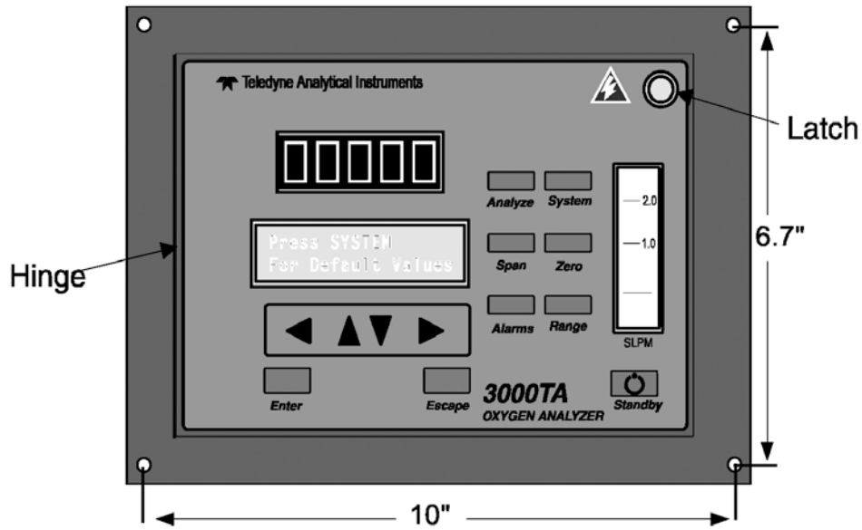
Figure 3-1: Front Panel of the Model 3000TA-EU
