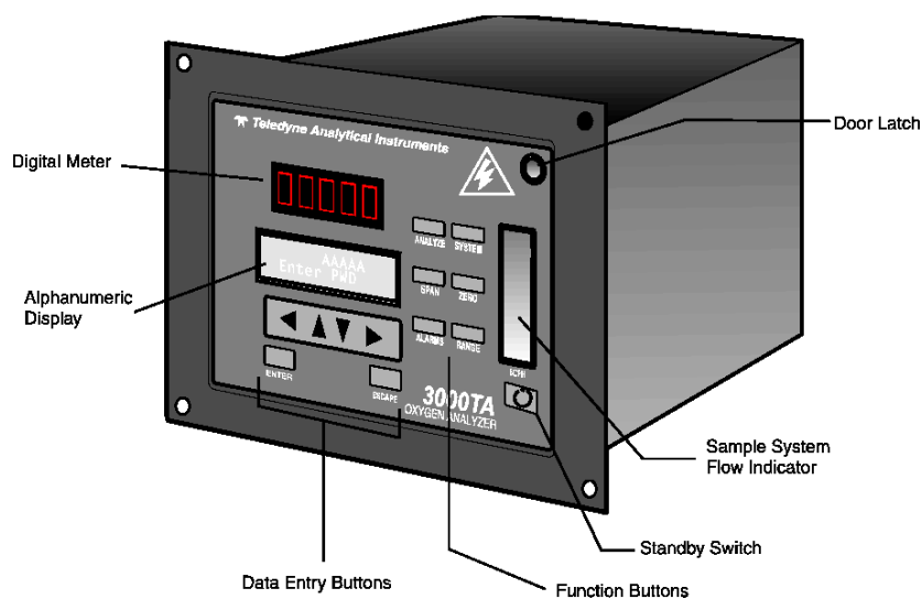
Figure 1-1: Model 3000TA-EU Front Panel
