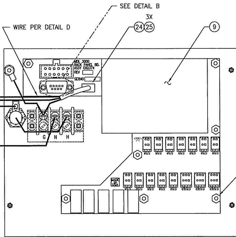
VIEW A-A REAR VIEW OF PC BOARD (ITEM 9)
